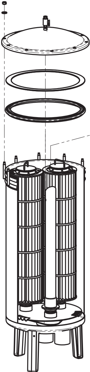
BF510 Exploded View
