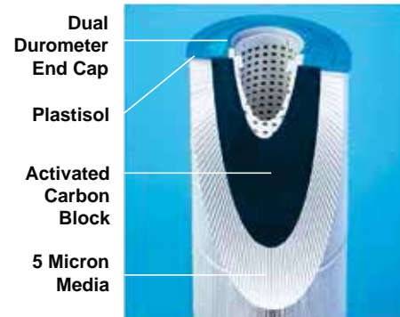
Cut-away view
