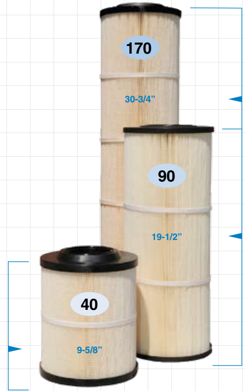
Hurricane® Cartridges Length and O.D.
